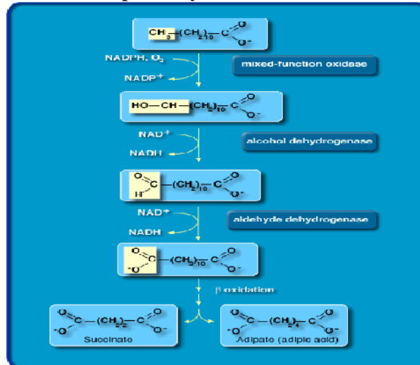
Figure 2.3: \omega -Oxidation pathway
