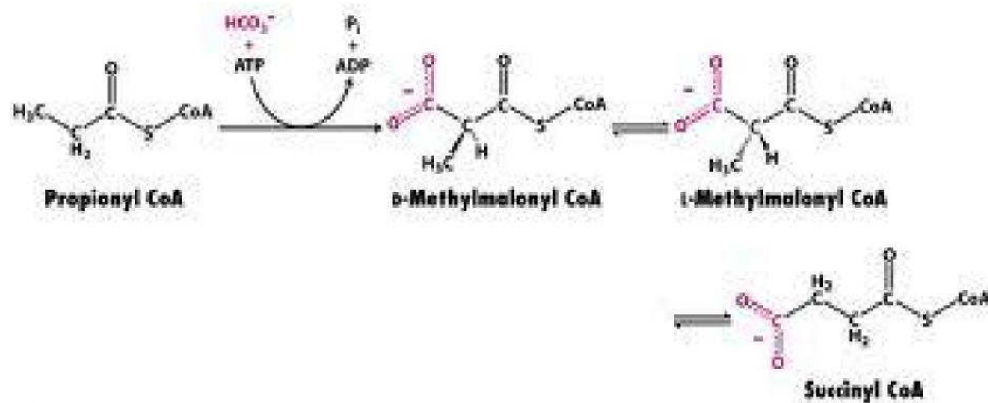
Figure 22-12 Biochemistry, Sixth Edition © 2013 W. H. Freeman and Company
