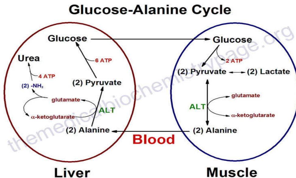
Figure: The glucose alanine cycle (© The medicalbiochemistrypage.org)
