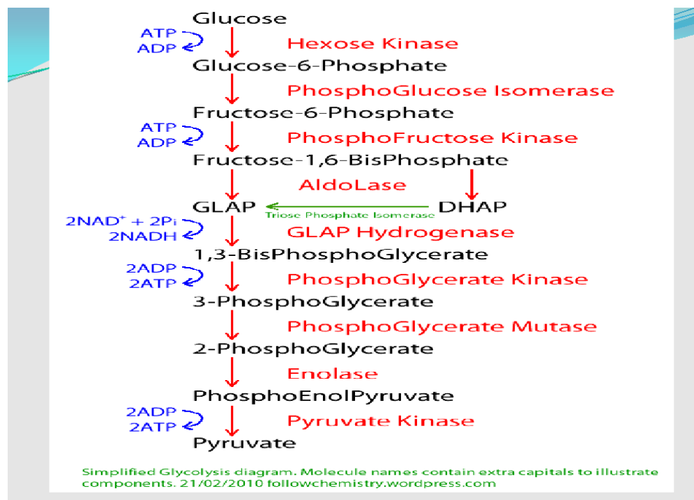
Fig 1.1: The Glycolytic Pathway
