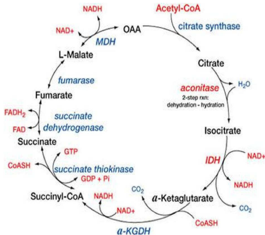
Figure 3.1: The TCA cycle showing the enzymes and the intermediates (source google images).
